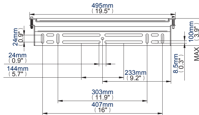
Wall Plate
